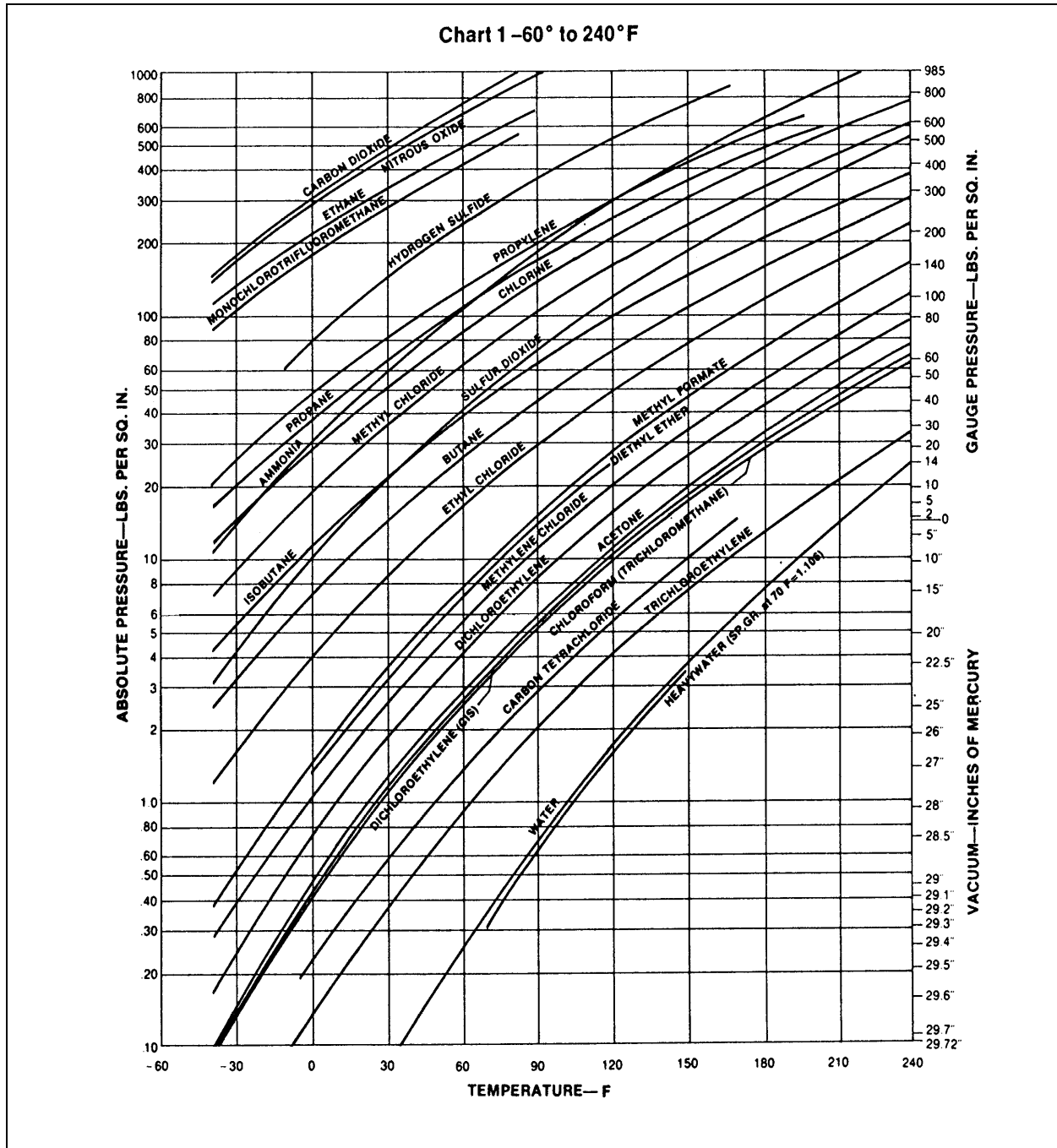
Fig. C-1 Vapor Pressure—Various Liquids (1 of 2) Courtesy of Goulds Pumps, Inc
