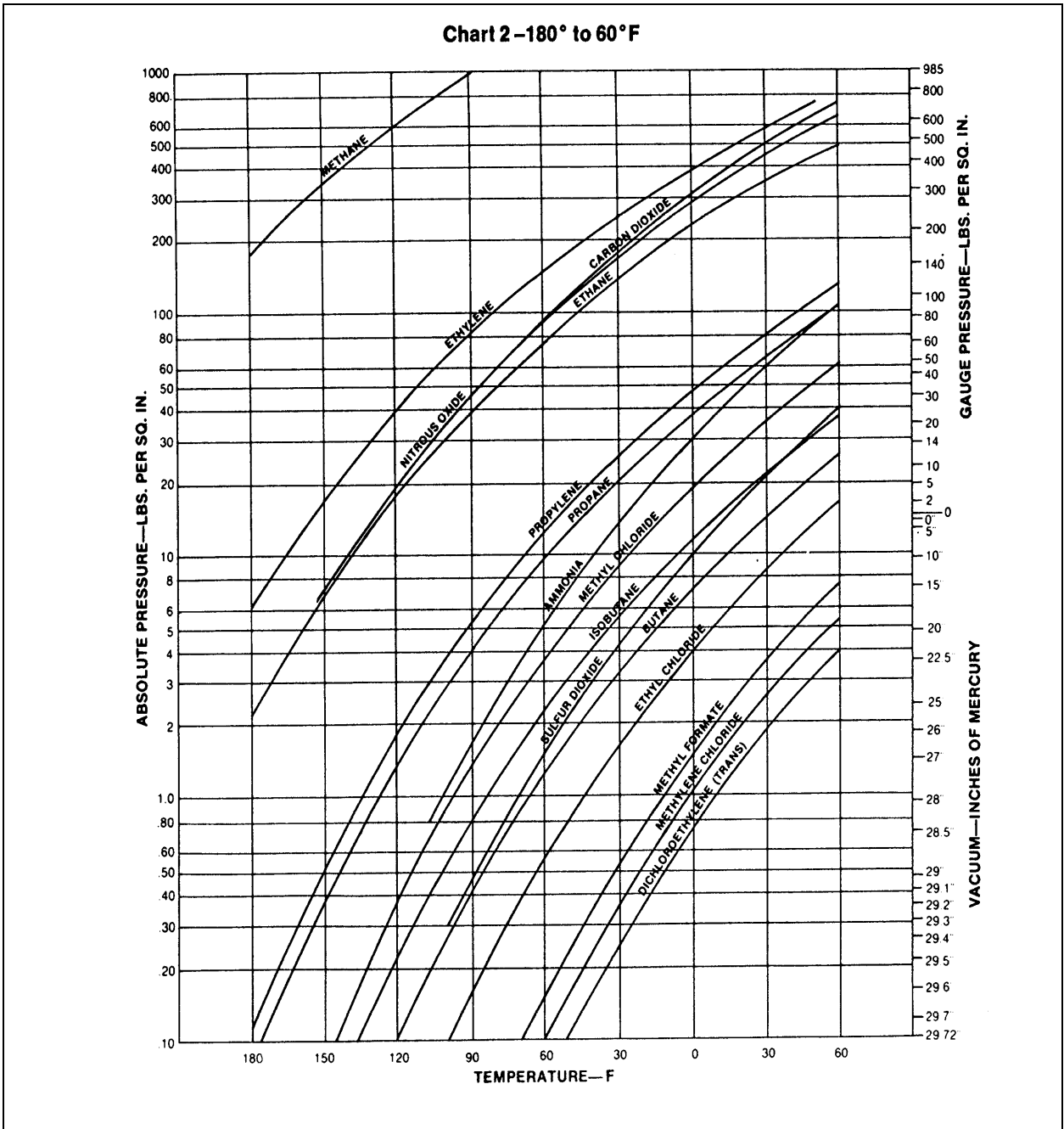
Fig. C-1 Vapor Pressure—Various Liquids (2 of 2) Courtesy of Goulds Pumps, Inc
