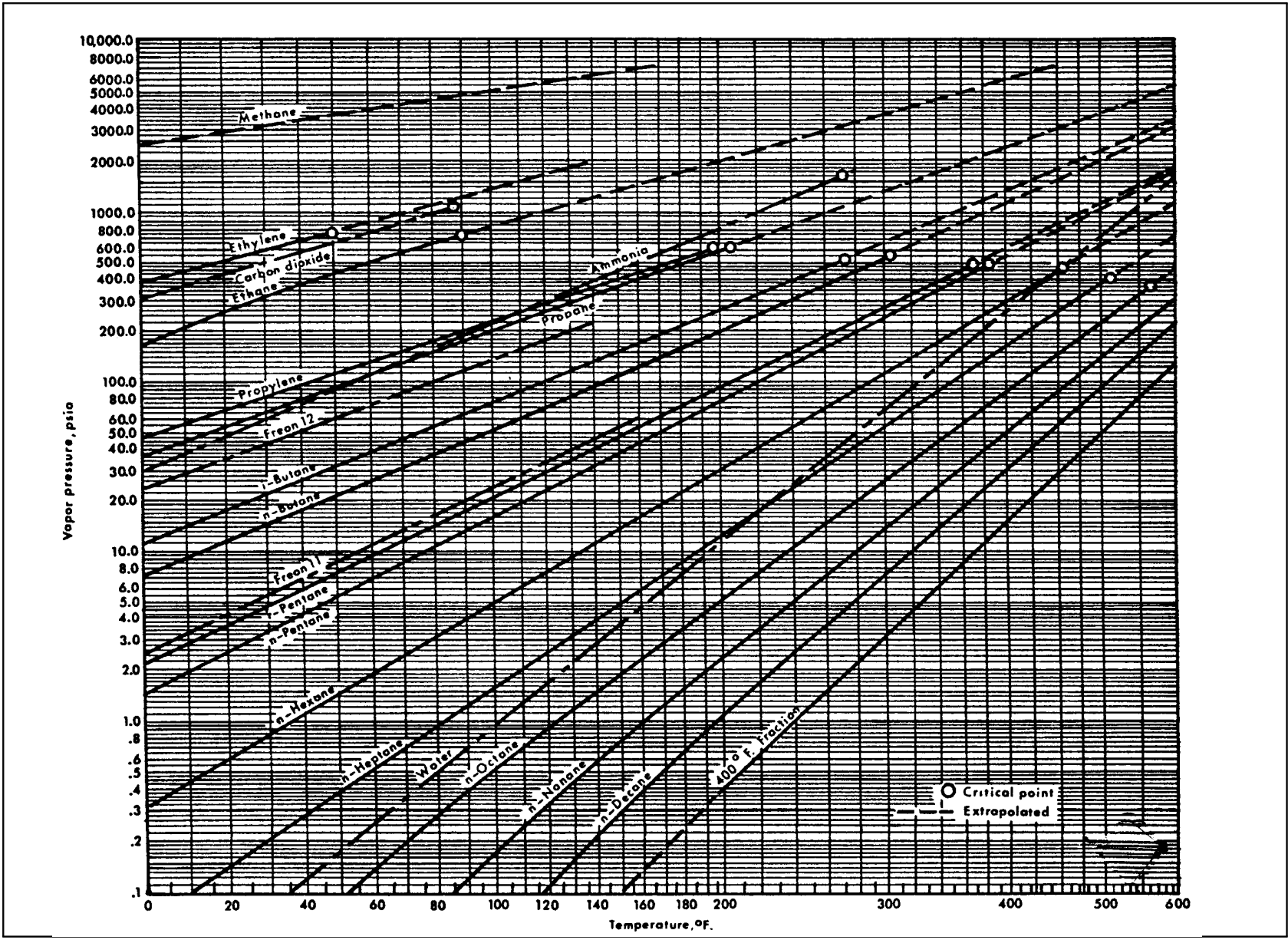
Fig. C-2 Low-Temperature Vapor Pressures for Light Hydrocarbons (2 of 2) Courtesy of GPSA
