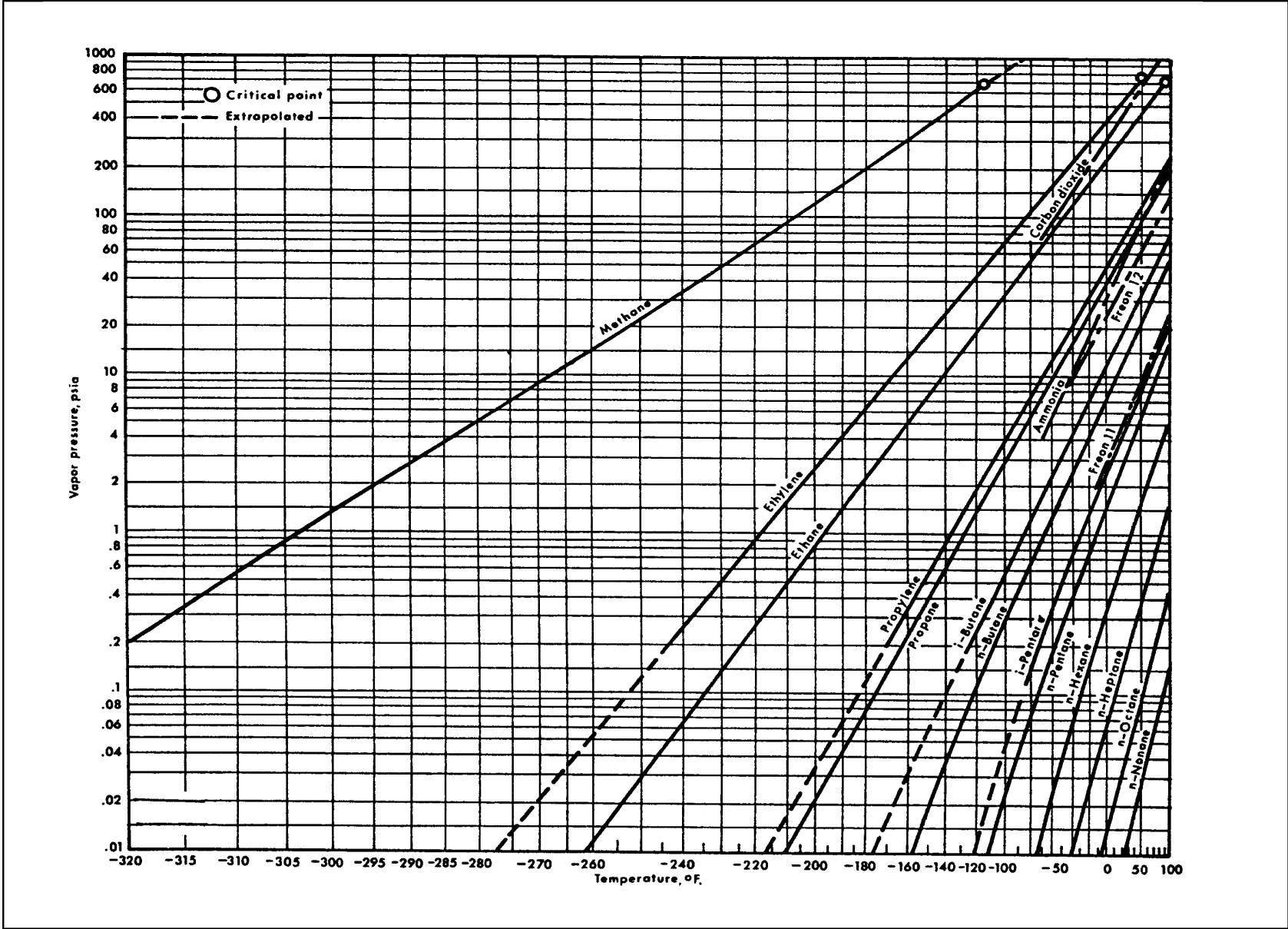
Fig. C-2 Low-Temperature Vapor Pressures for Light Hydrocarbons (1 of 2) Courtesy of GPSA
